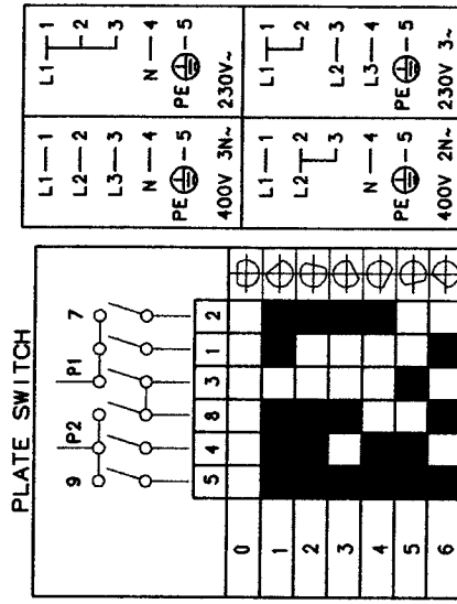
WIRING DIAGRAM
