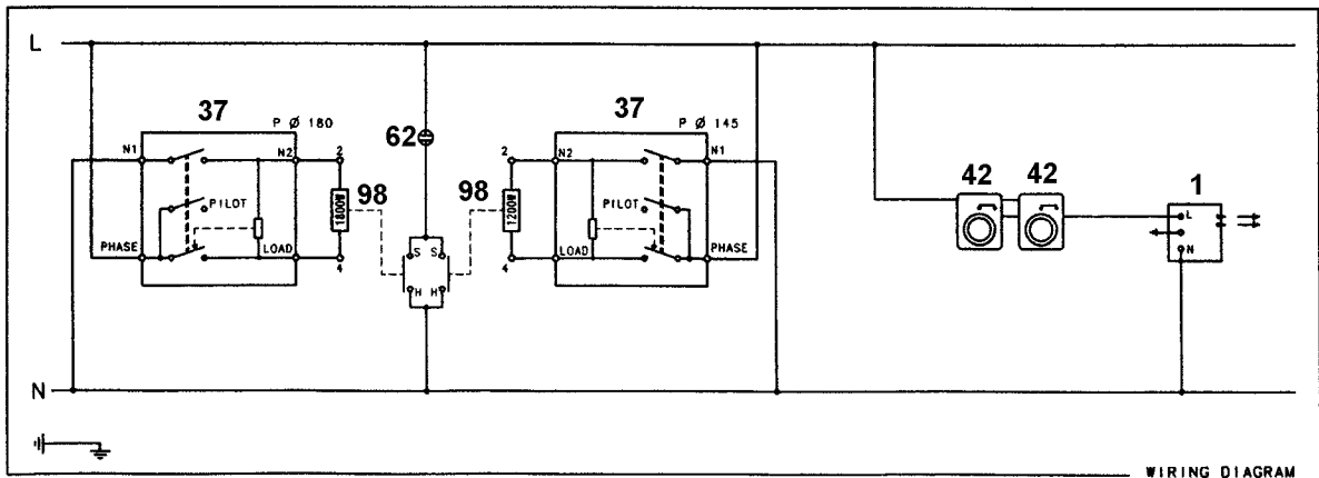
WIRING DIAGRAM
