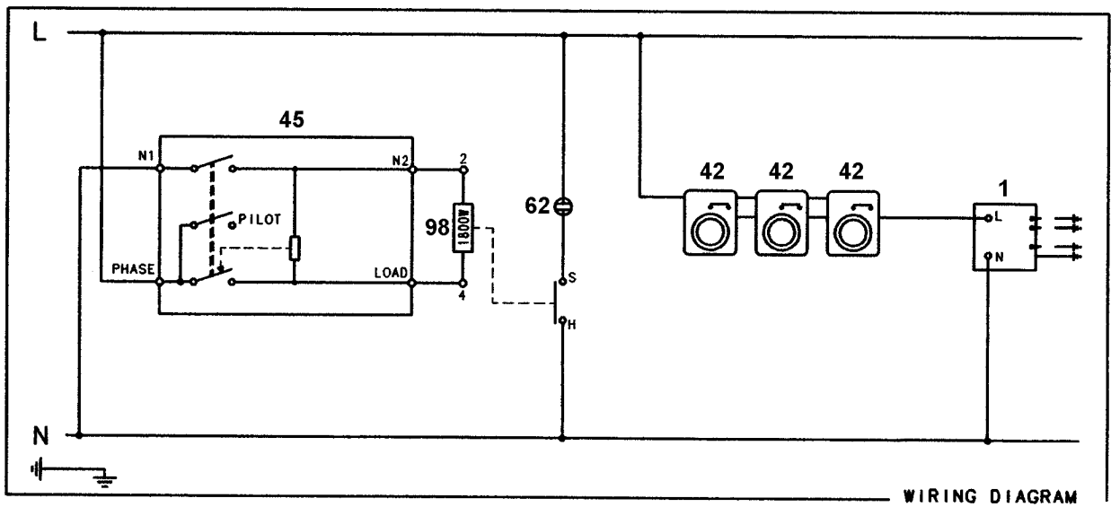
WIRING DIAGRAM
