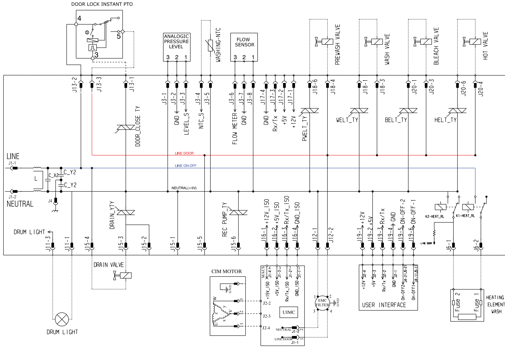
ELECTRIC DIAGRAM EWX11
