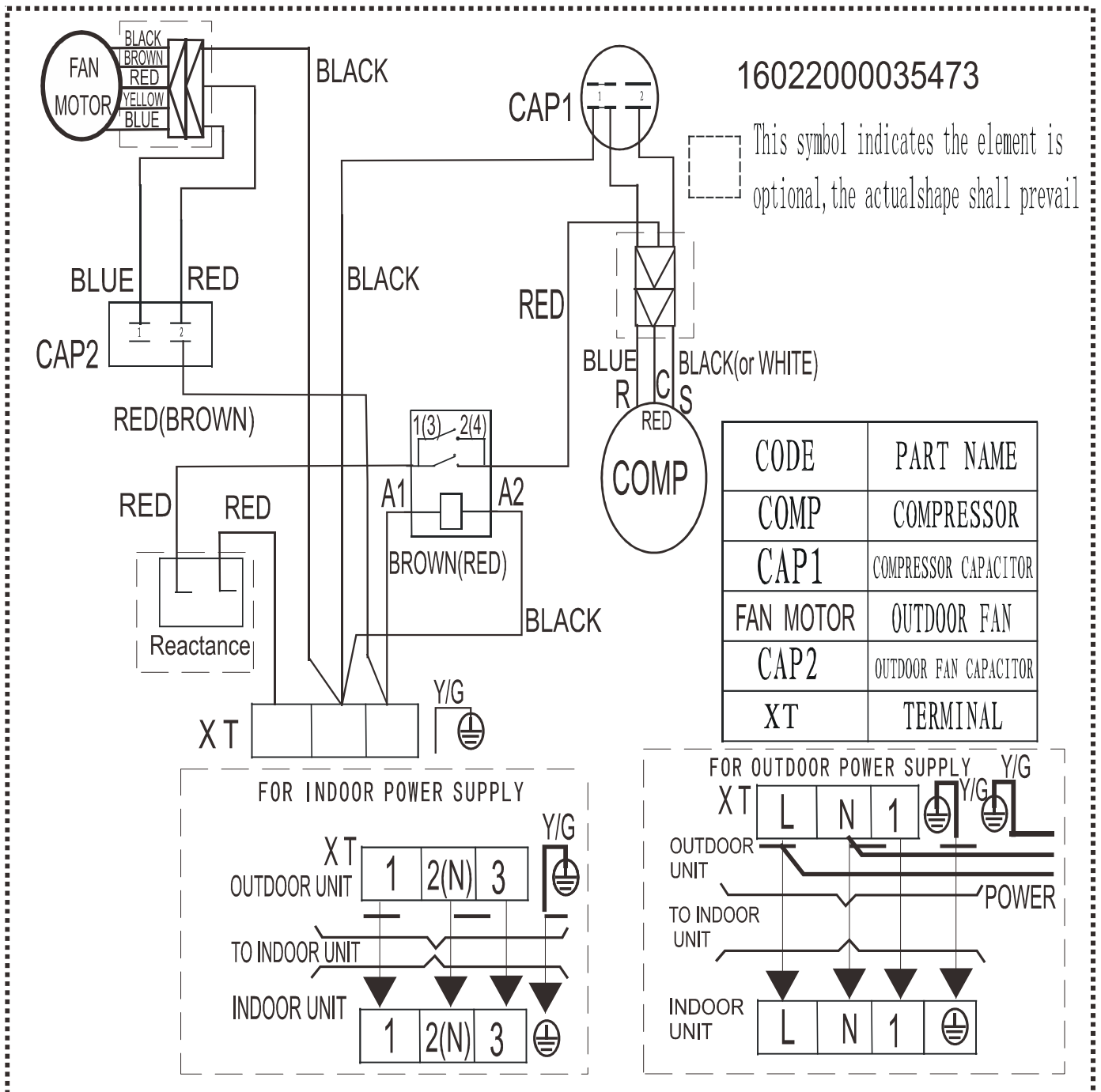
Outdoor unit wiring diagram: 16022000035473
