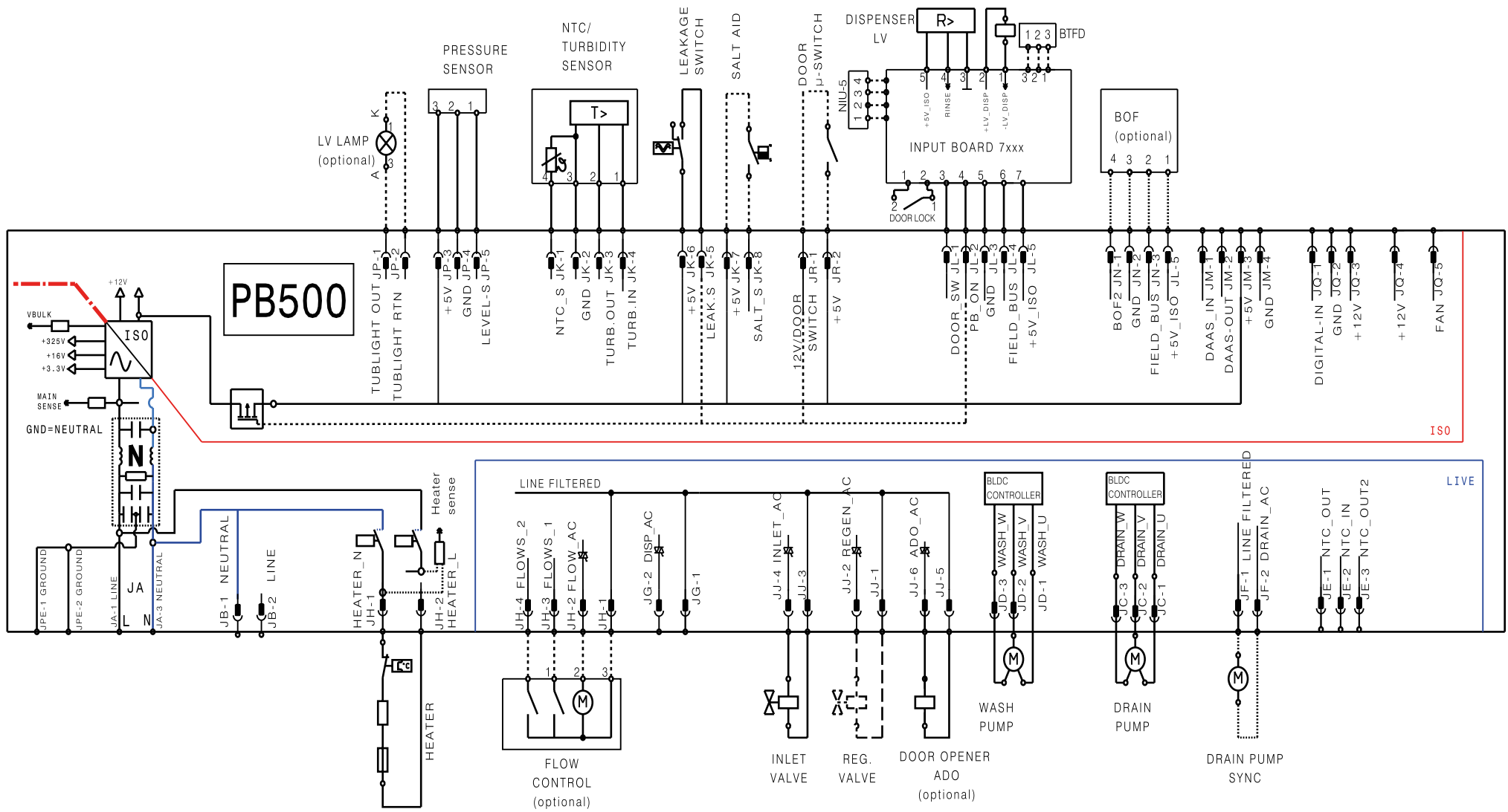
ELECTRONIC DIAGRAM PB500
