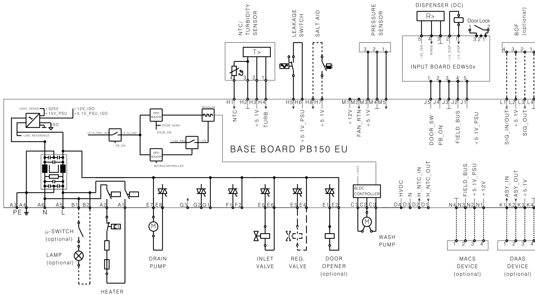
CIRCUIT DIAGRAM
