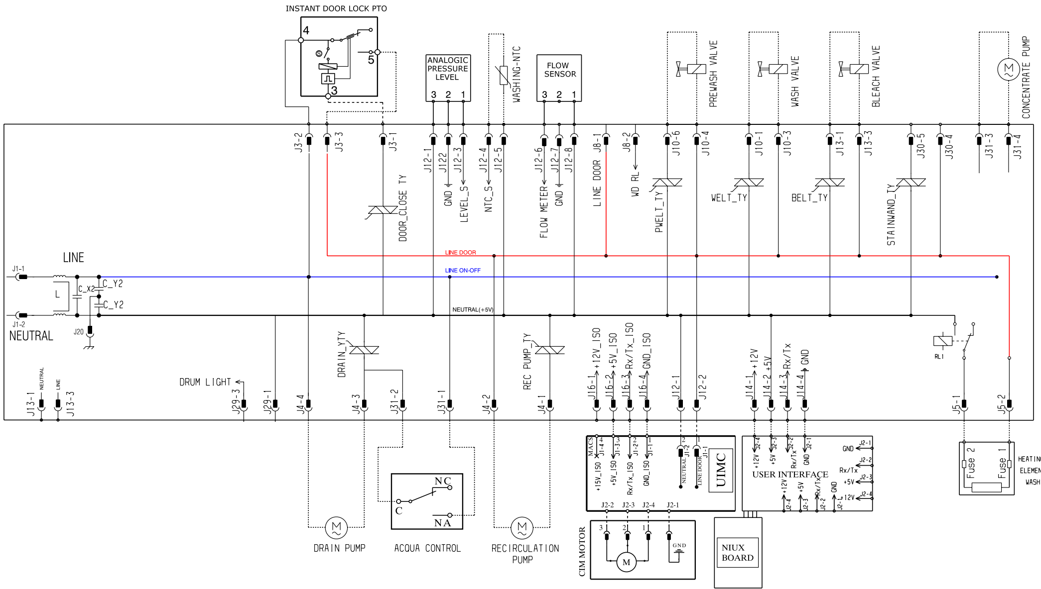
ELECTRIC DIAGRAM EVWX14
