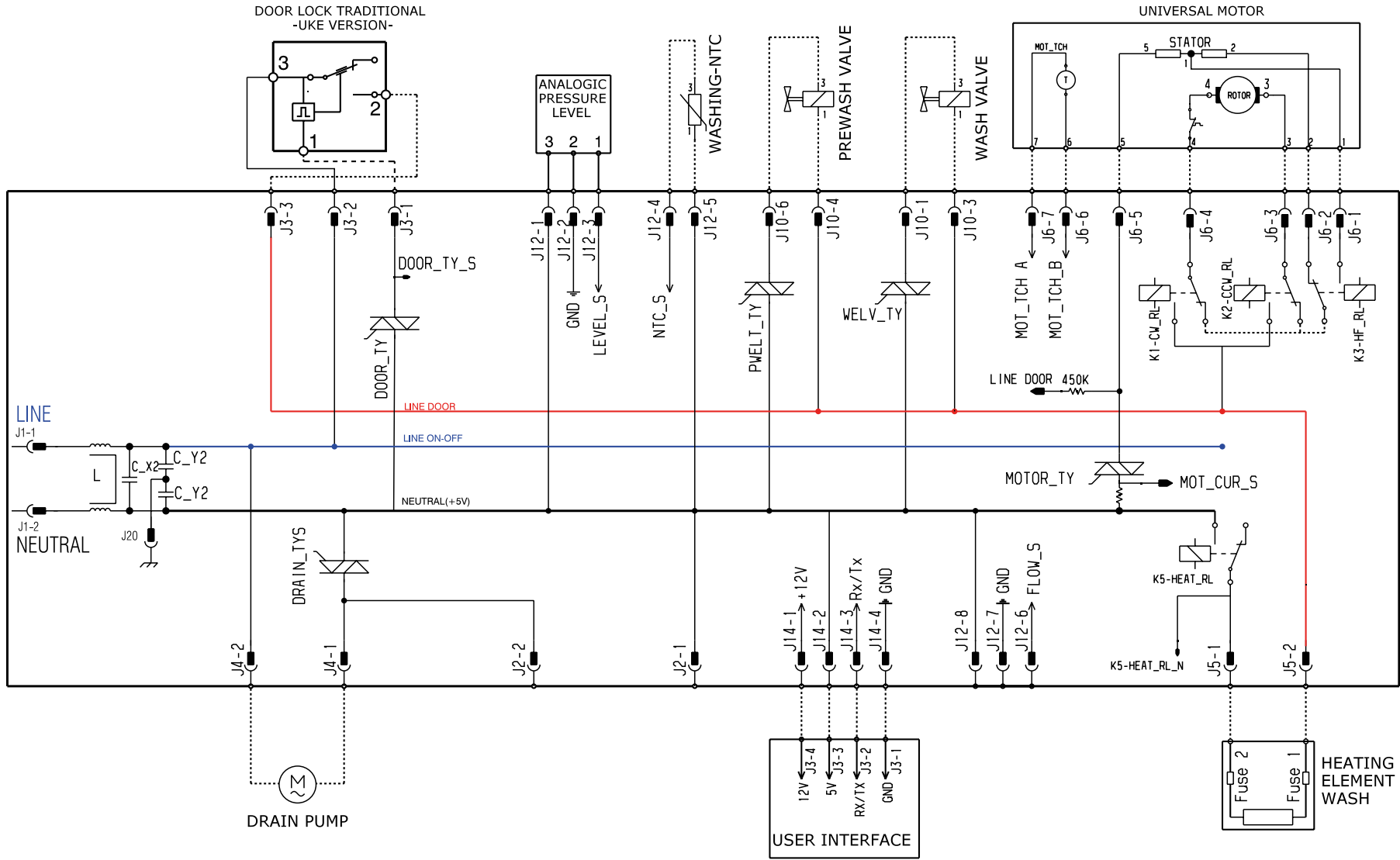
ELECTRIC DIAGRAM -EWX 13-
