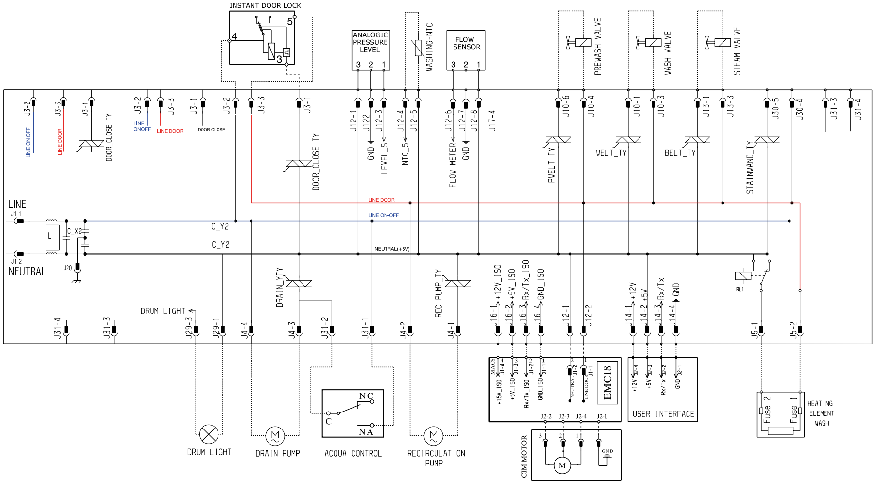
ELECTRIC DIAGRAM EWX14
