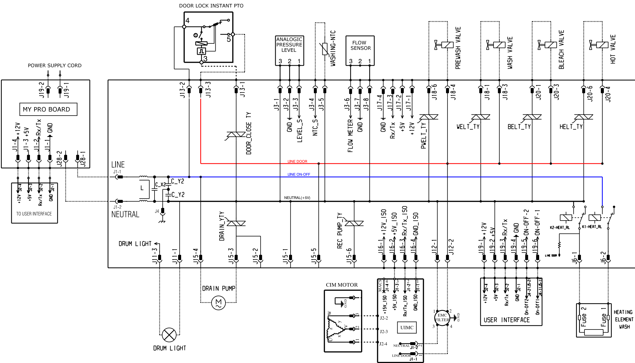
ELECTRIC DIAGRAM EWX11
