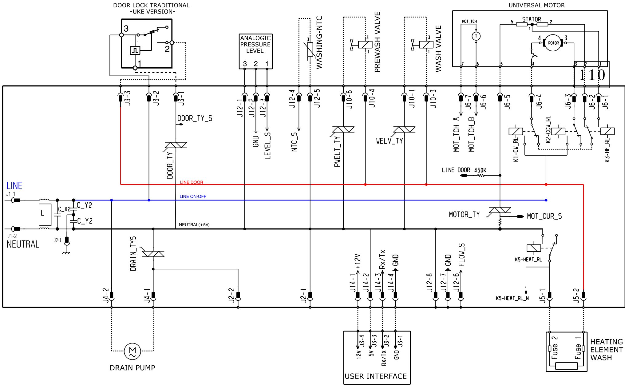
ELECTRIC DIAGRAM -EWX 13-
