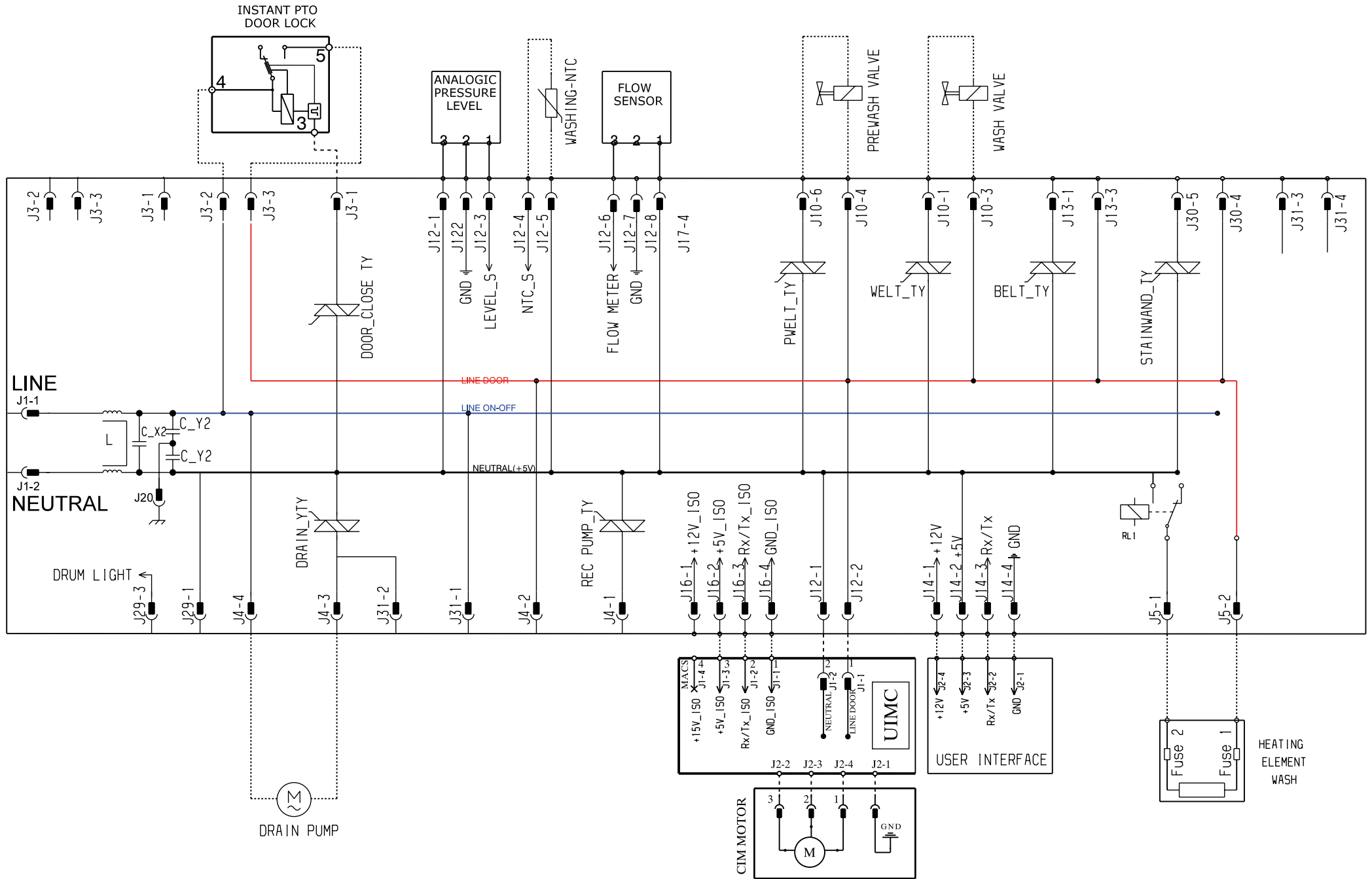
ELECTRIC DIAGRAM EWX14
