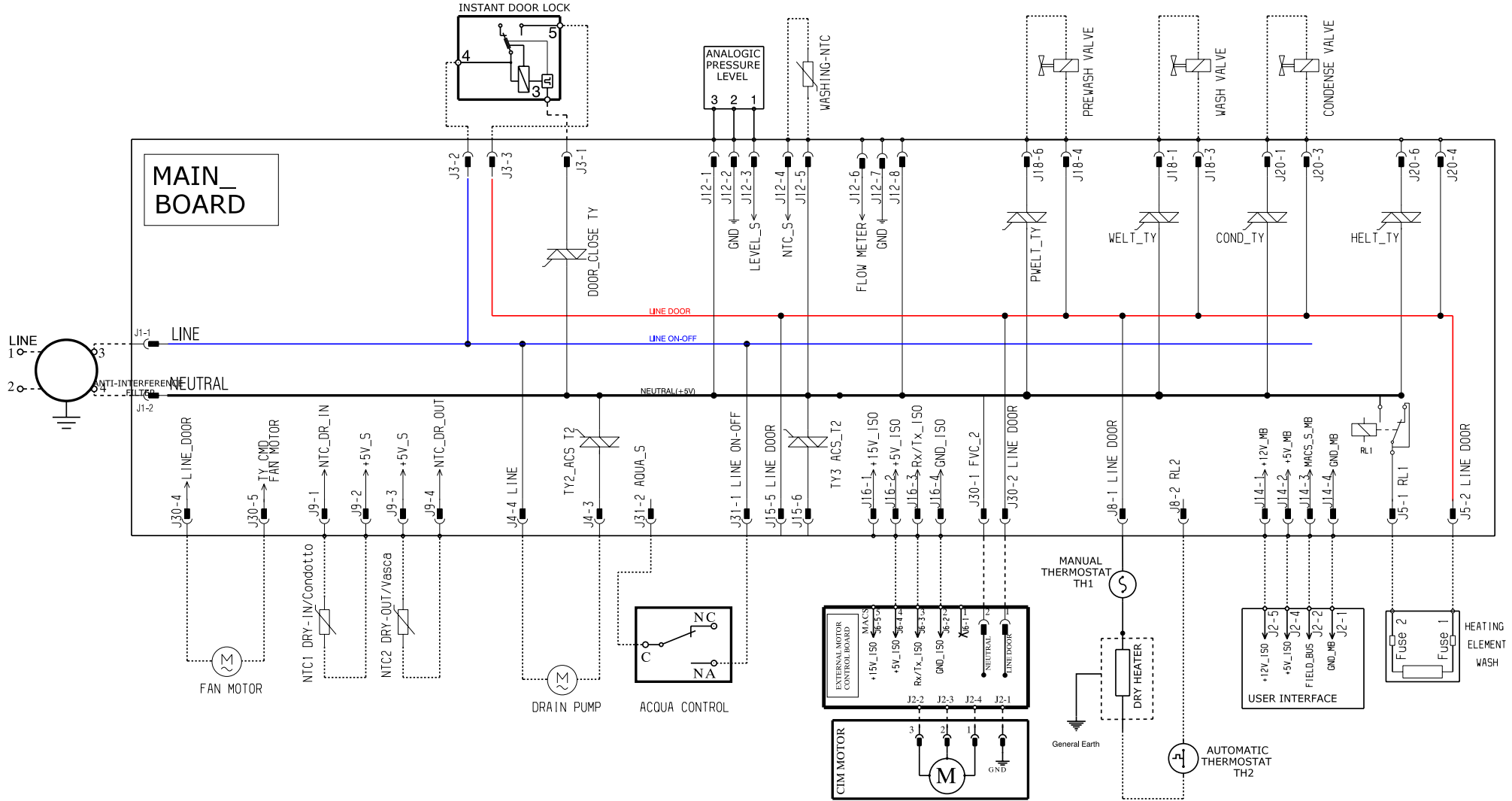
ELECTRIC DIAGRAM EWX14 WD
