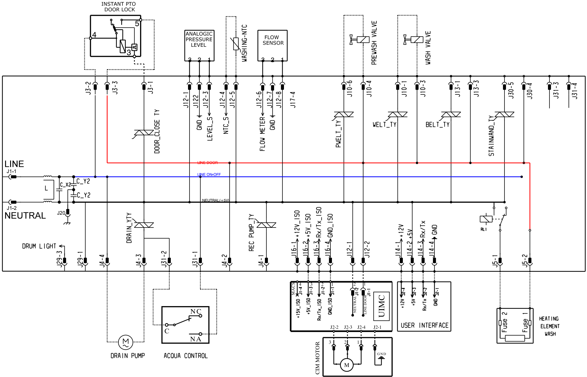
ELECTRIC DIAGRAM EWX14
