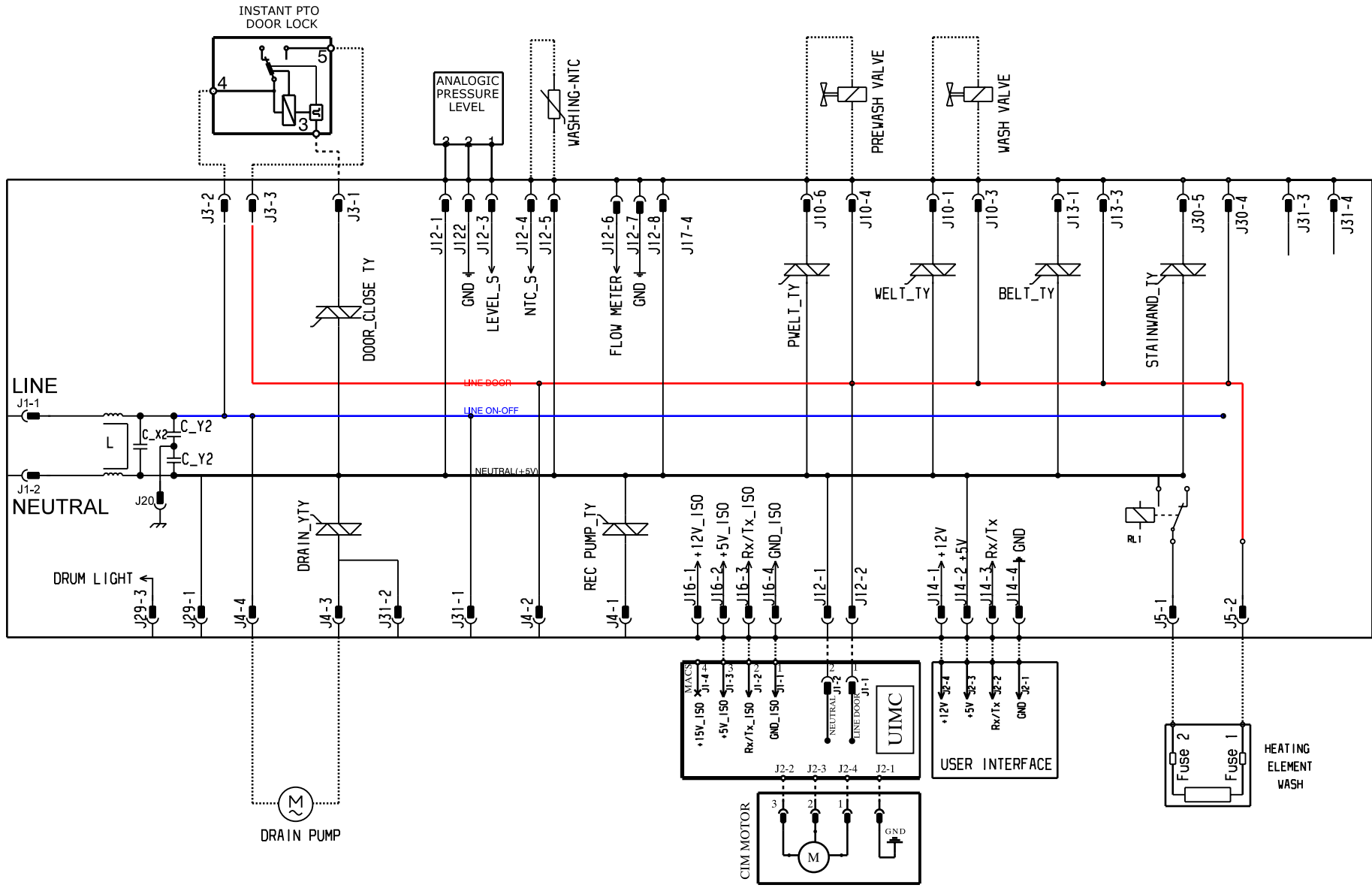
ELECTRIC DIAGRAM EWX14
