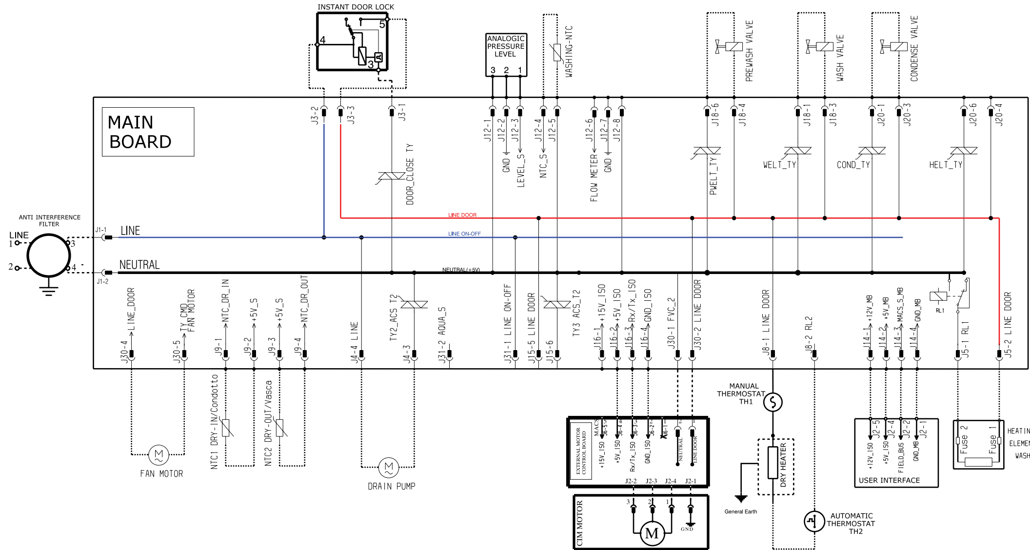
ELECTRIC DIAGRAM EWX14 WD
