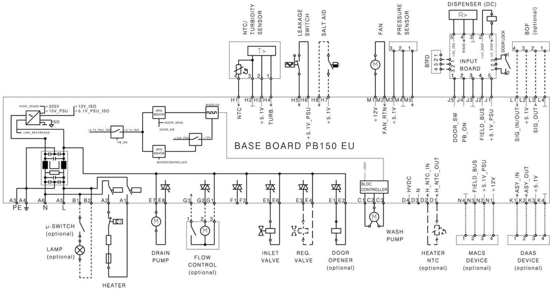
CIRCUIT DIAGRAM
