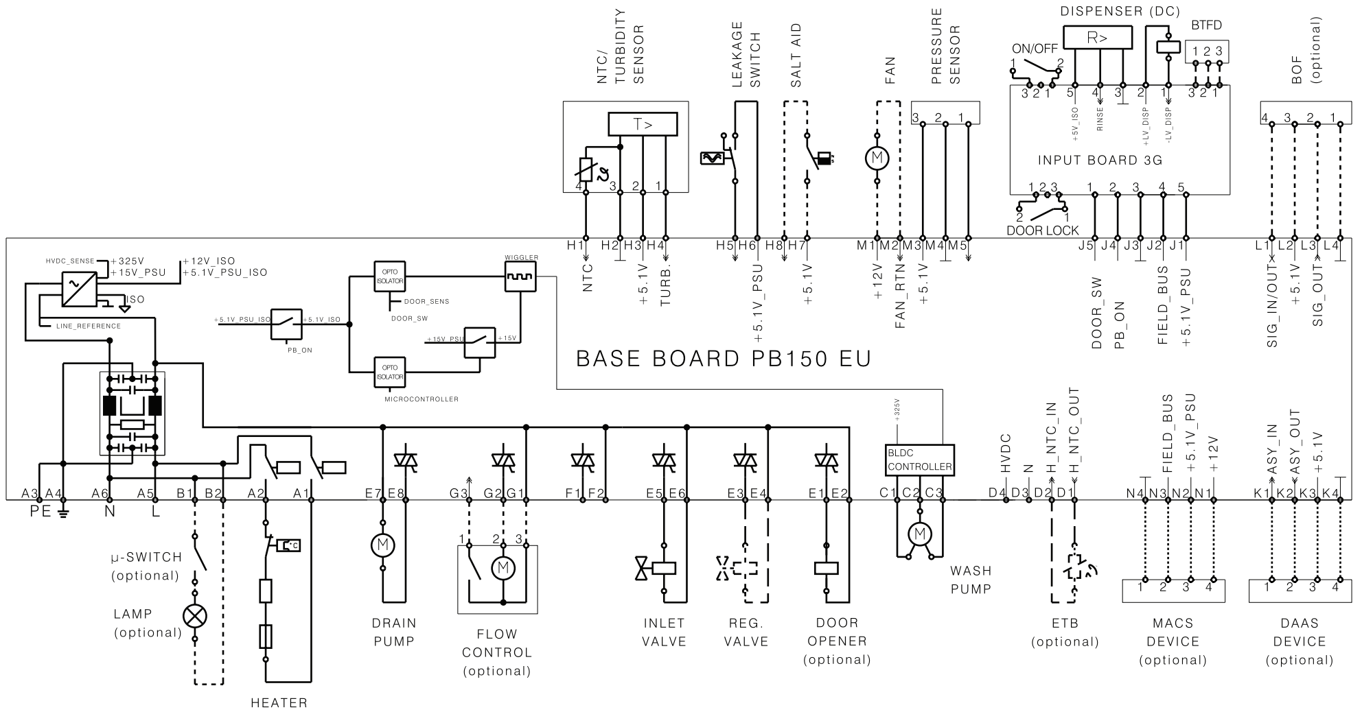
CIRCUIT DIAGRAM
