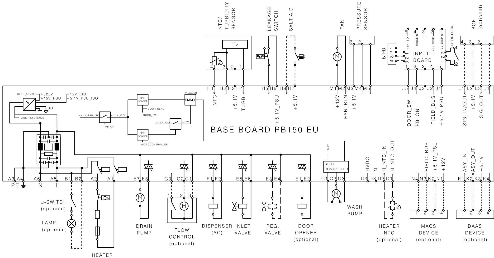
CIRCUIT DIAGRAM
