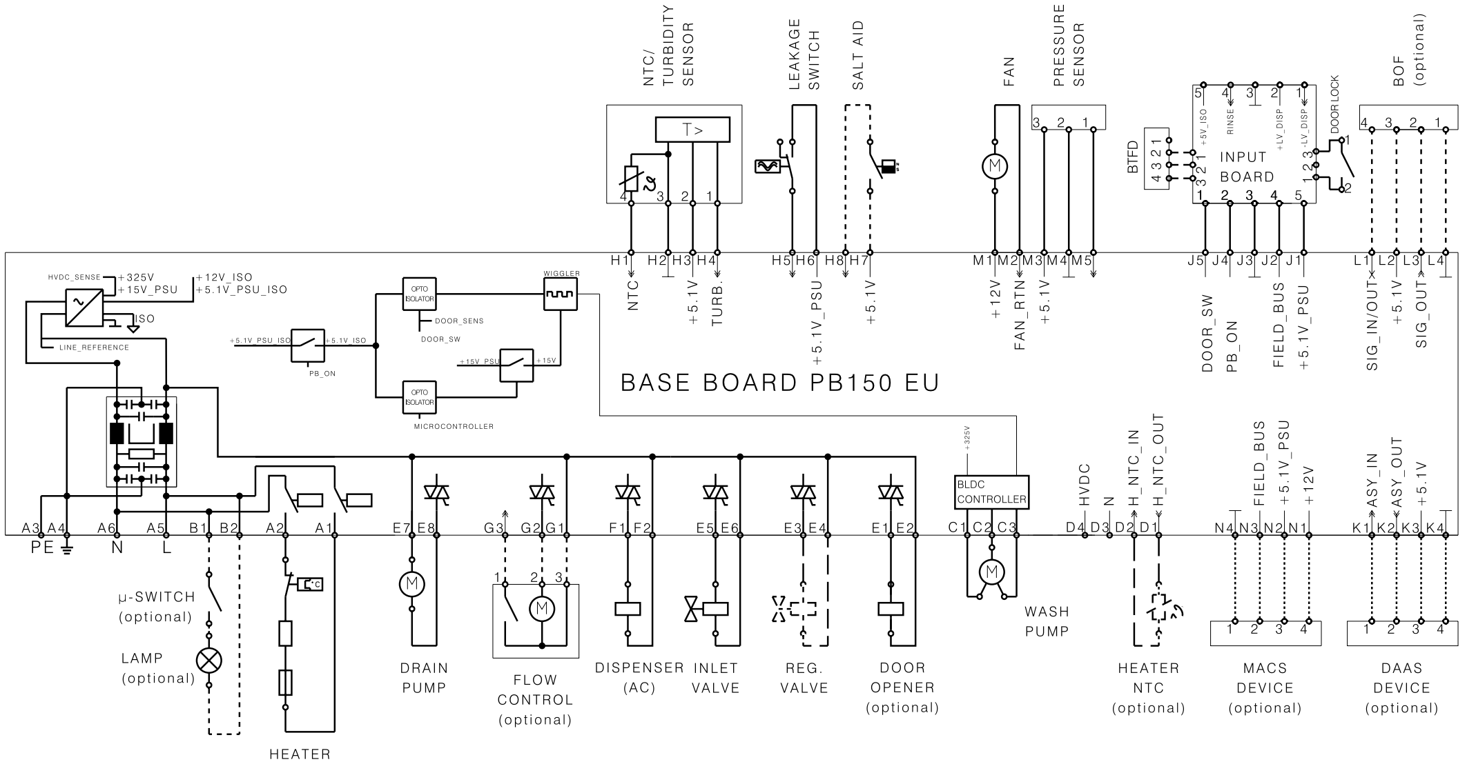
CIRCUIT DIAGRAM
