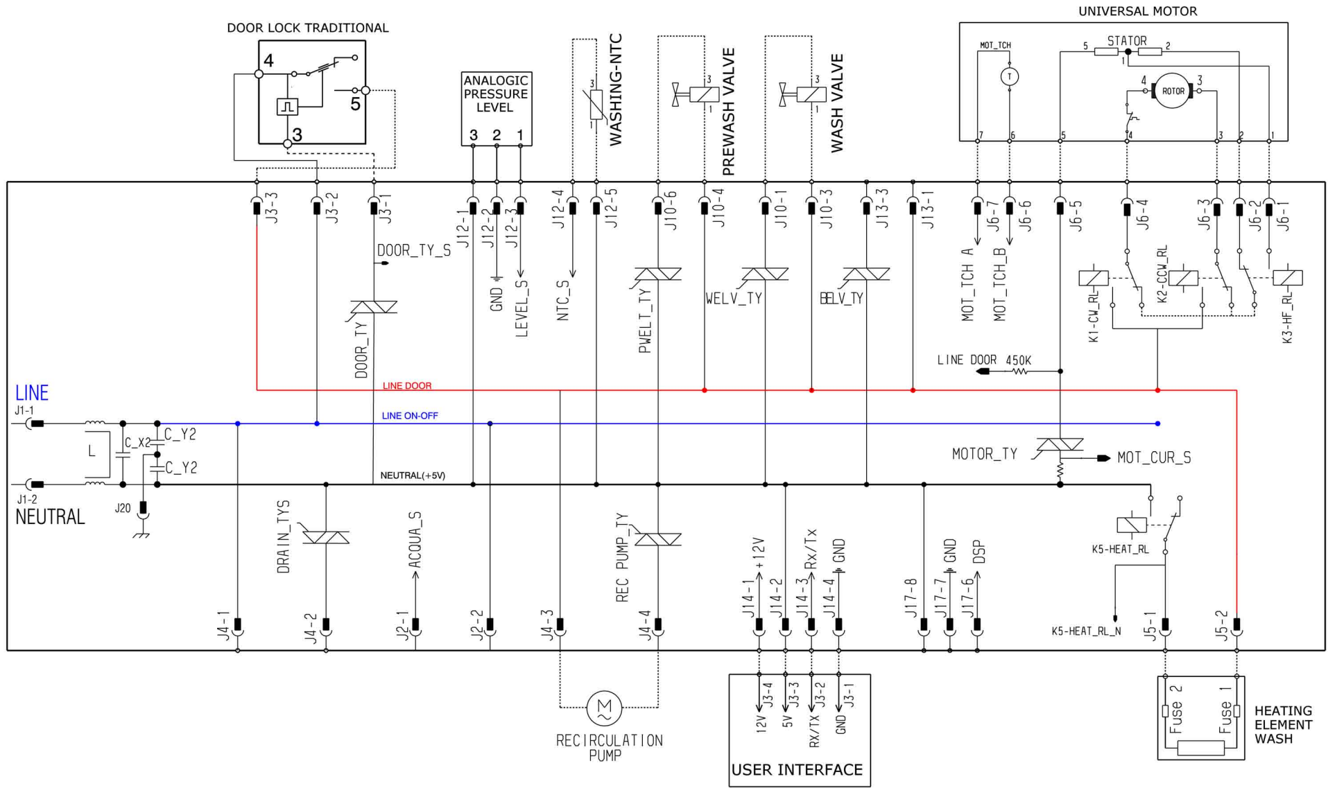
ELECTRIC DIAGRAM -EWX 13-
