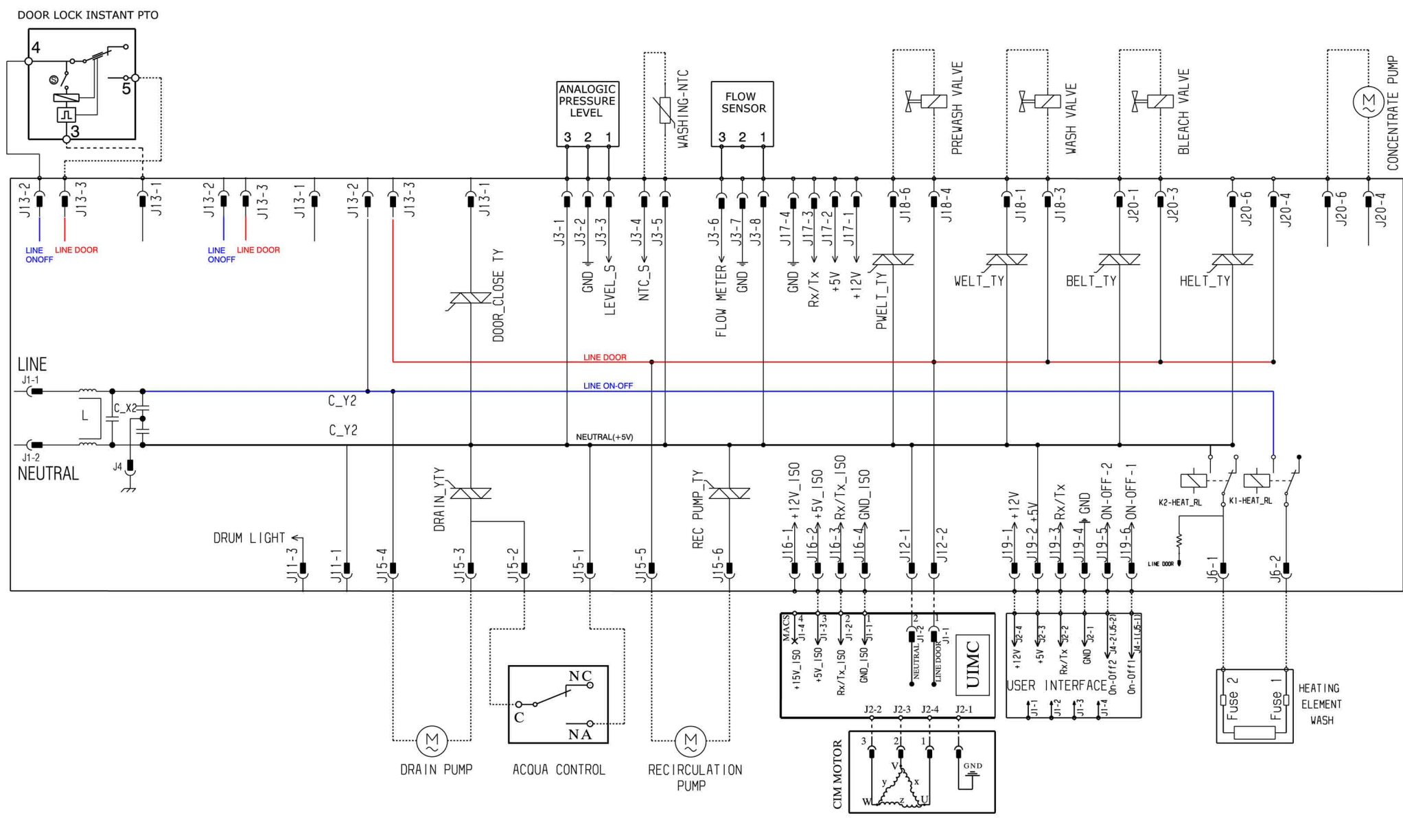
ELECTRIC DIAGRAM EWX11
