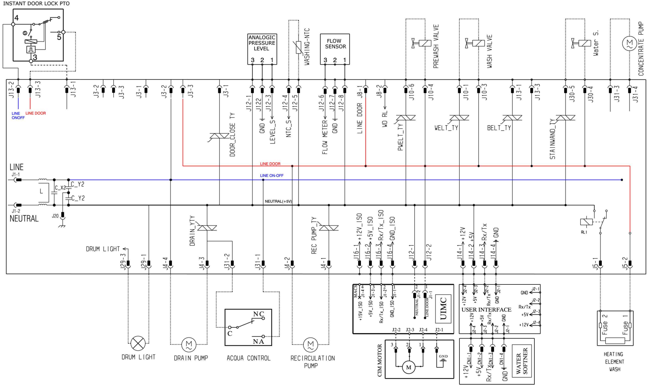
ELECTRIC DIAGRAM EWX14
