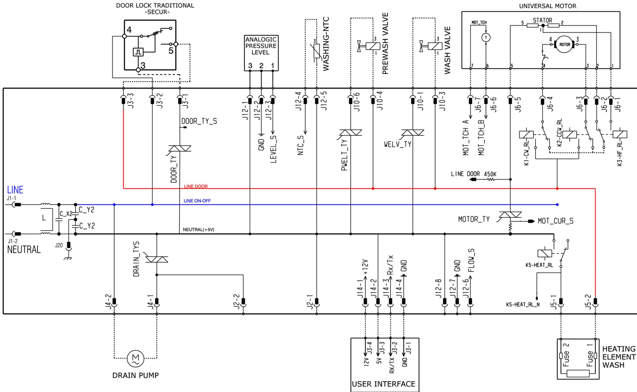
ELECTRIC DIAGRAM -EWX 13-
