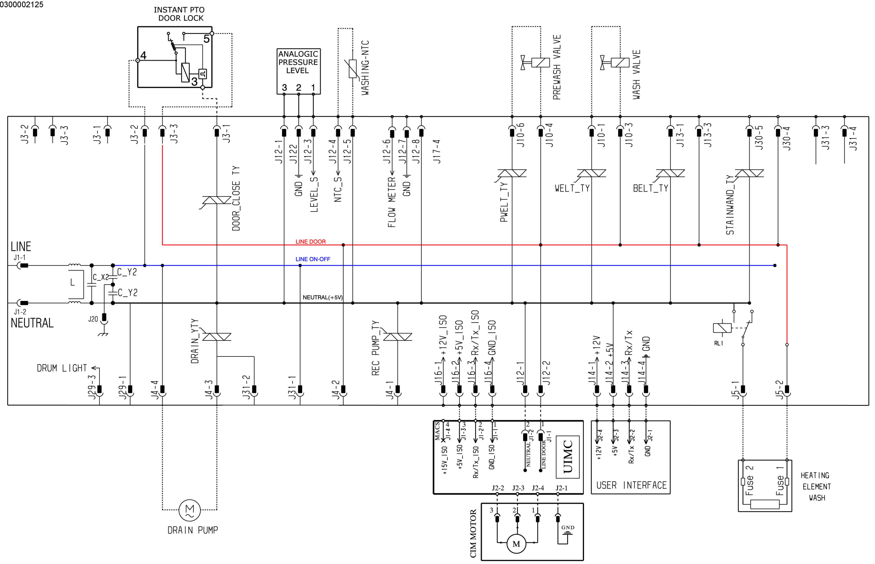
ELECTRIC DIAGRAM EWX14
