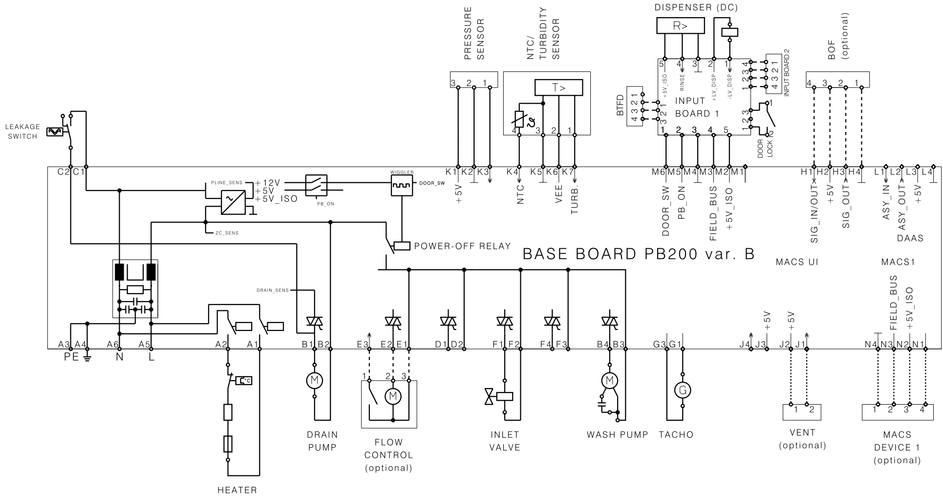
CIRCUIT DIAGRAM
