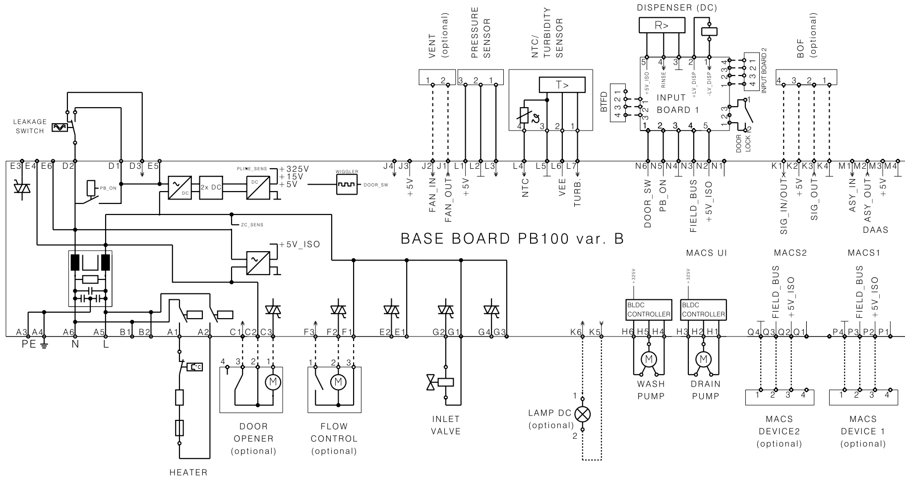
CIRCUIT DIAGRAM
