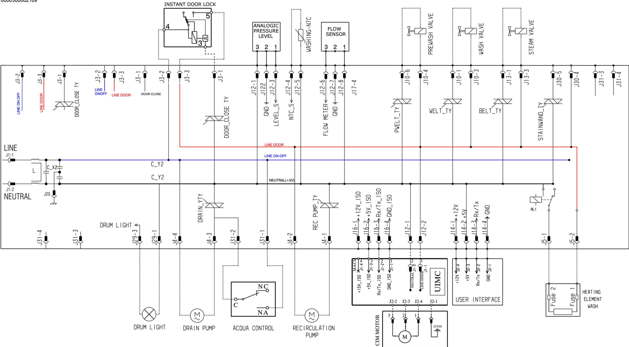
ELECTRIC DIAGRAM EWX14
