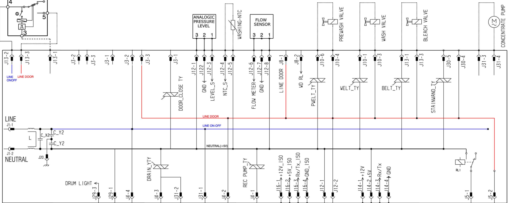
ELECTRIC DIAGRAM EWX14
