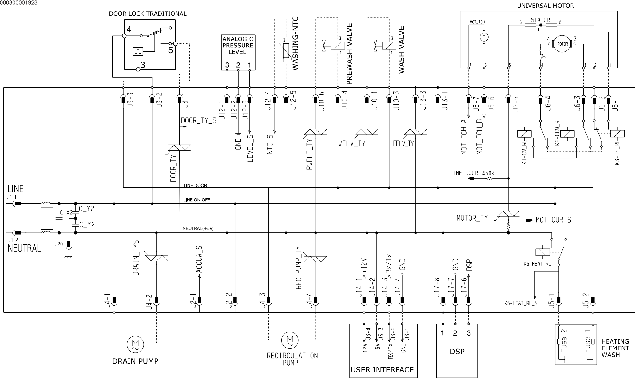
ELECTRIC DIAGRAM -EWX 13-
