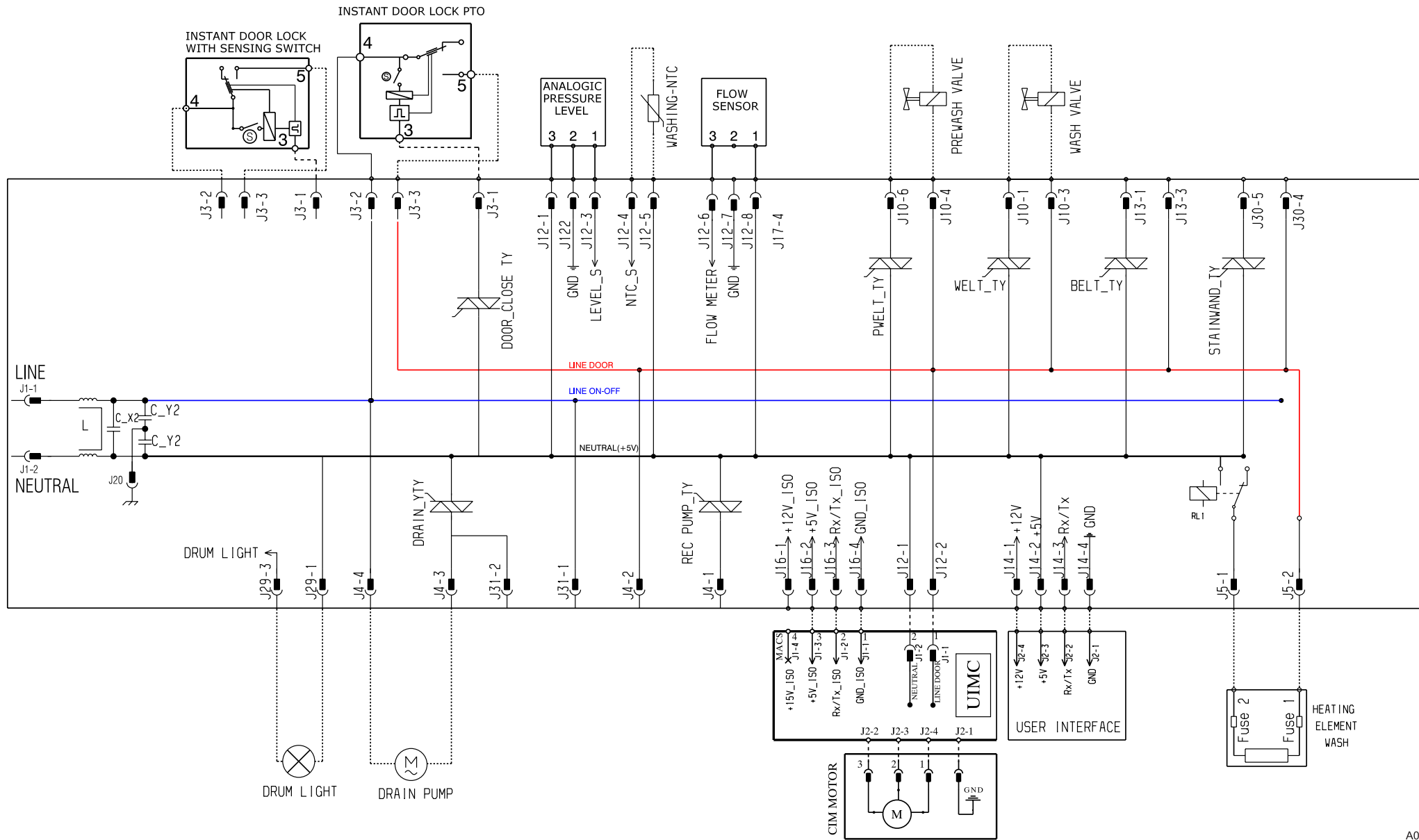
ELECTRIC DIAGRAM EWX14
