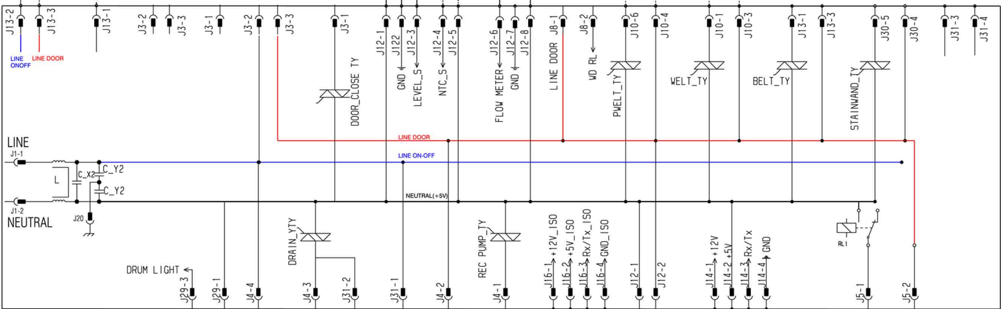
ELECTRIC DIAGRAM EWX14
