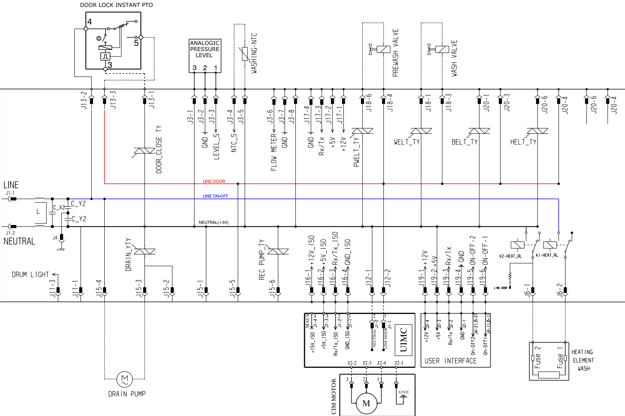
ELECTRIC DIAGRAM EWX11
