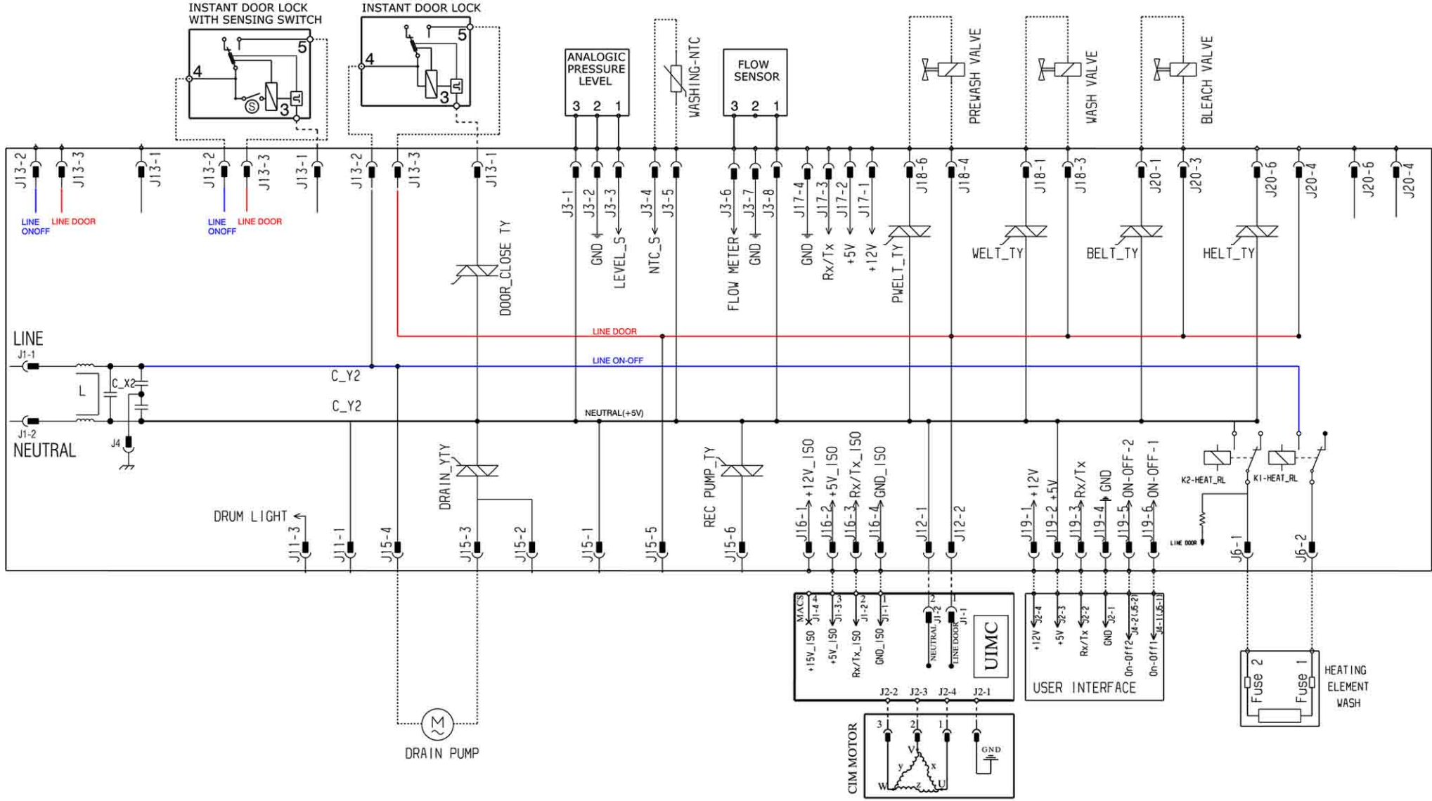
ELECTRIC DIAGRAM EWX11
