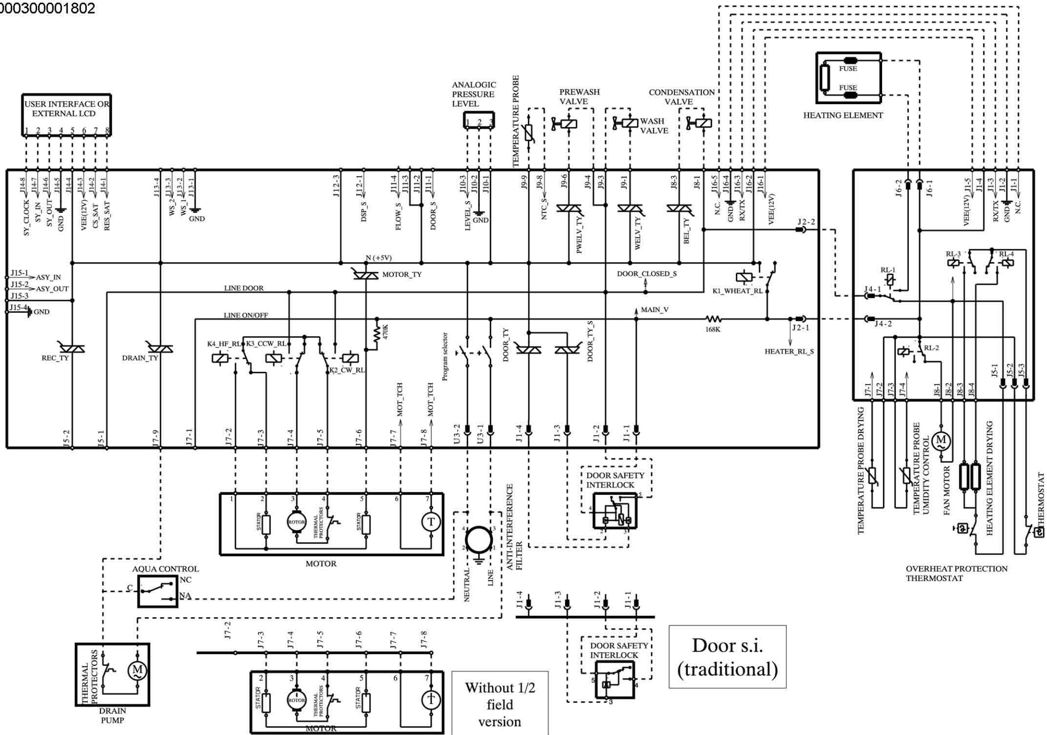
ELECTRIC DIAGRAM
