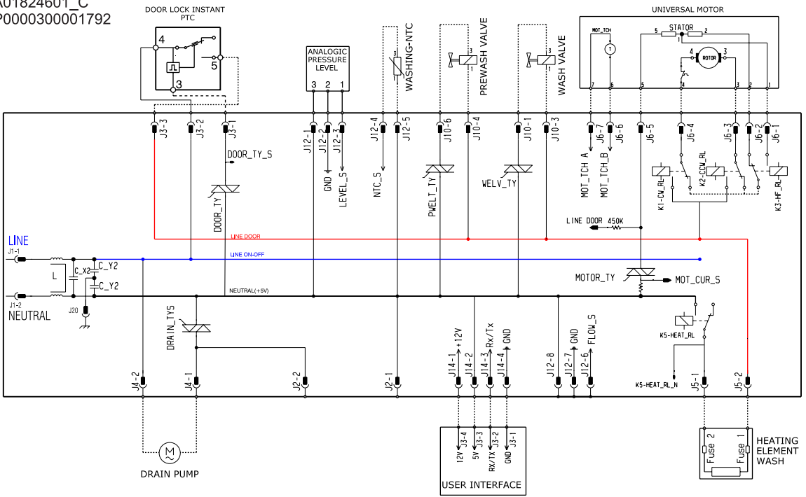
ELECTRIC DIAGRAM -EWX 13-
