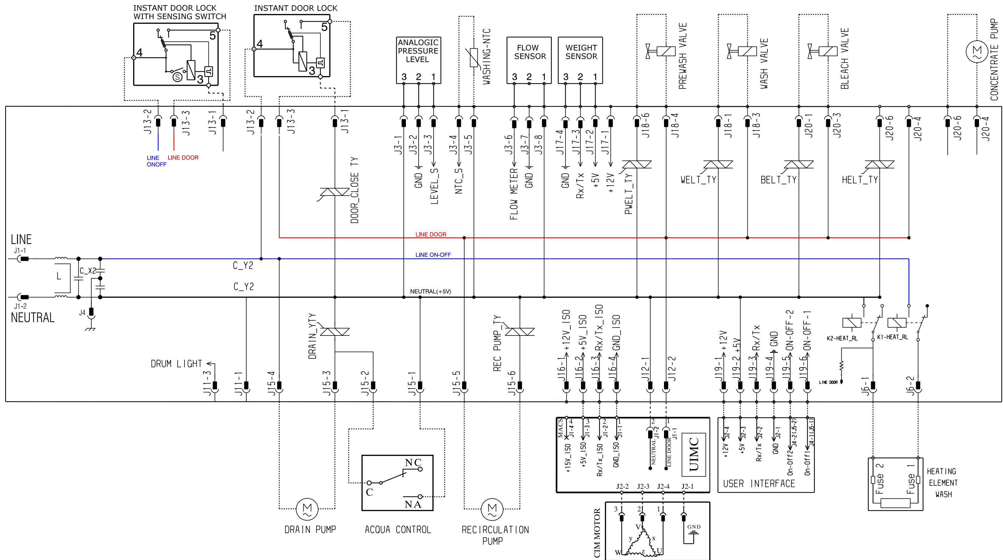
ELECTRIC DIAGRAM EWX11
