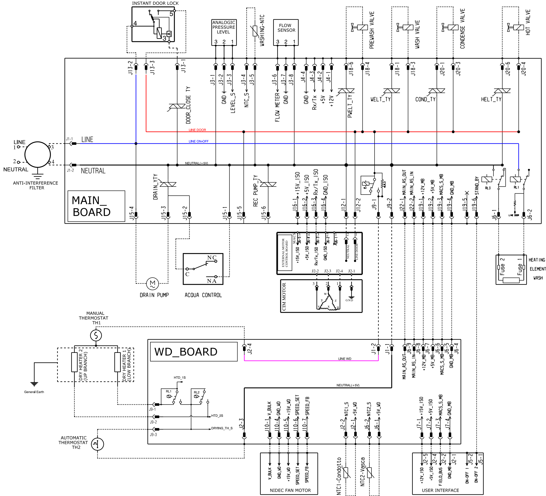
ELECTRIC DIAGRAM EWX11 WD
