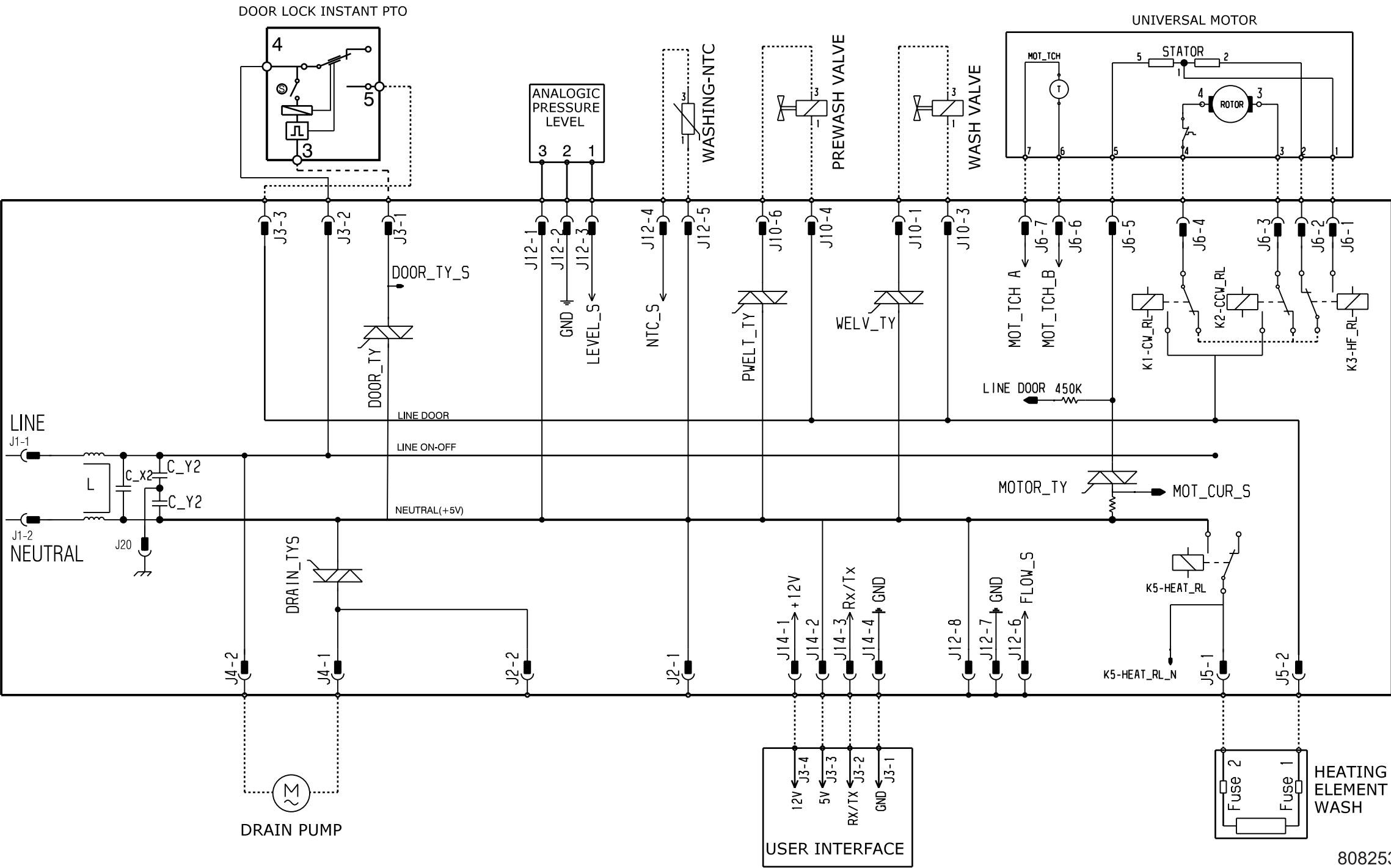
ELECTRIC DIAGRAM -EWX 13-
