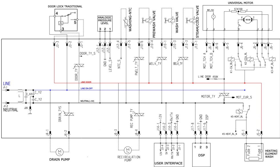
ELECTRIC DIAGRAM -EWX 13-
