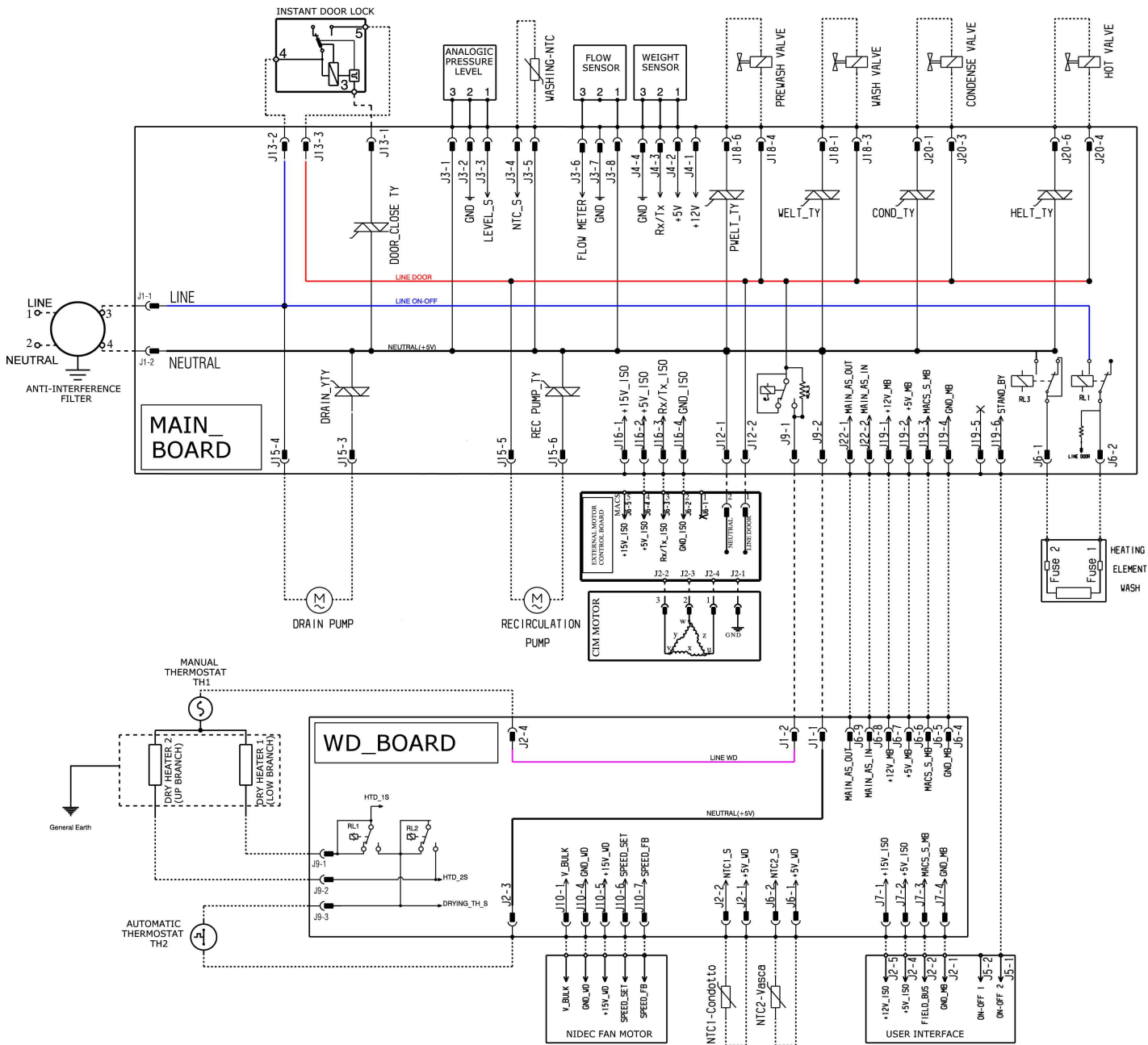
ELECTRIC DIAGRAM EWX11 WD
