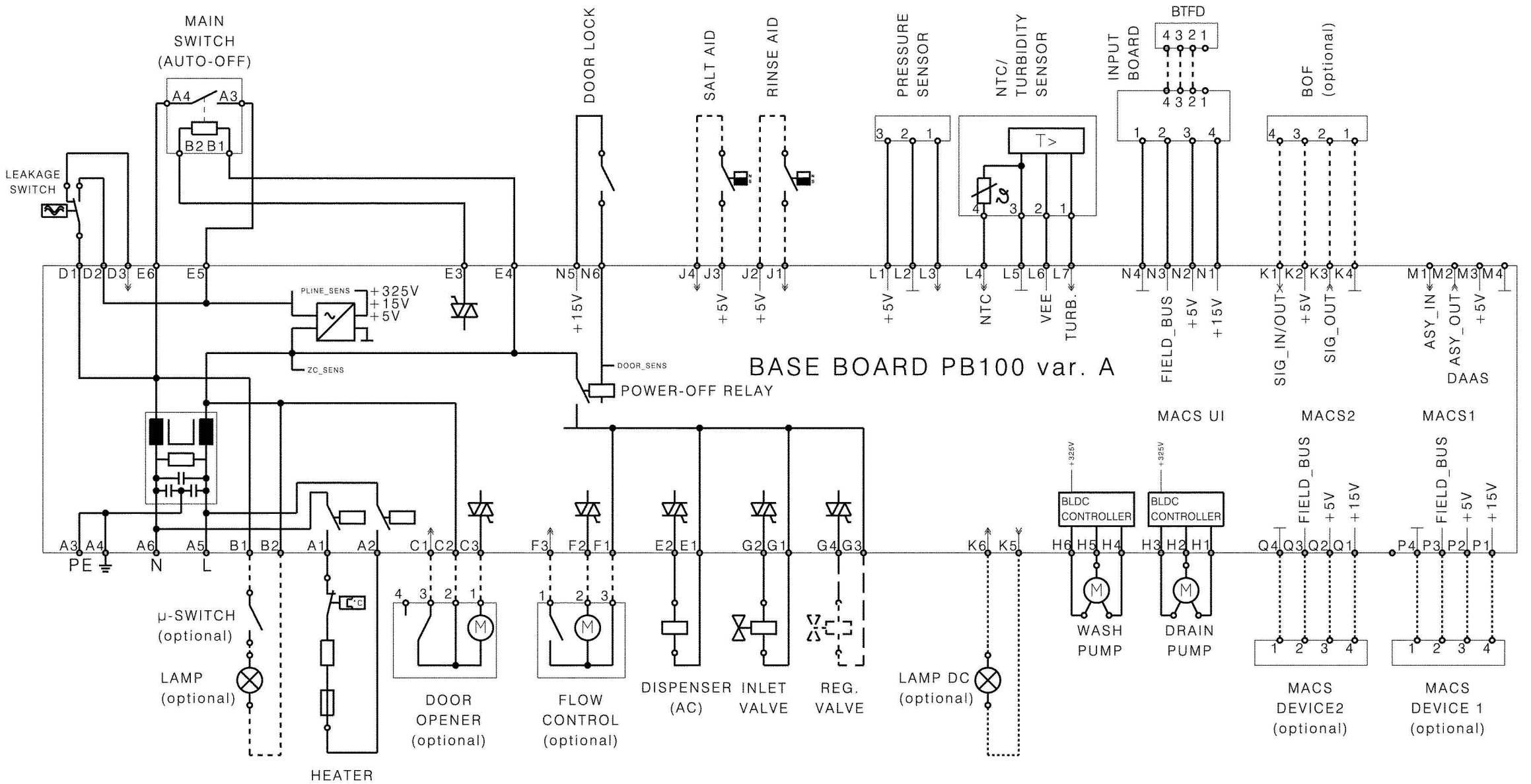
CIRCUIT DIAGRAM
