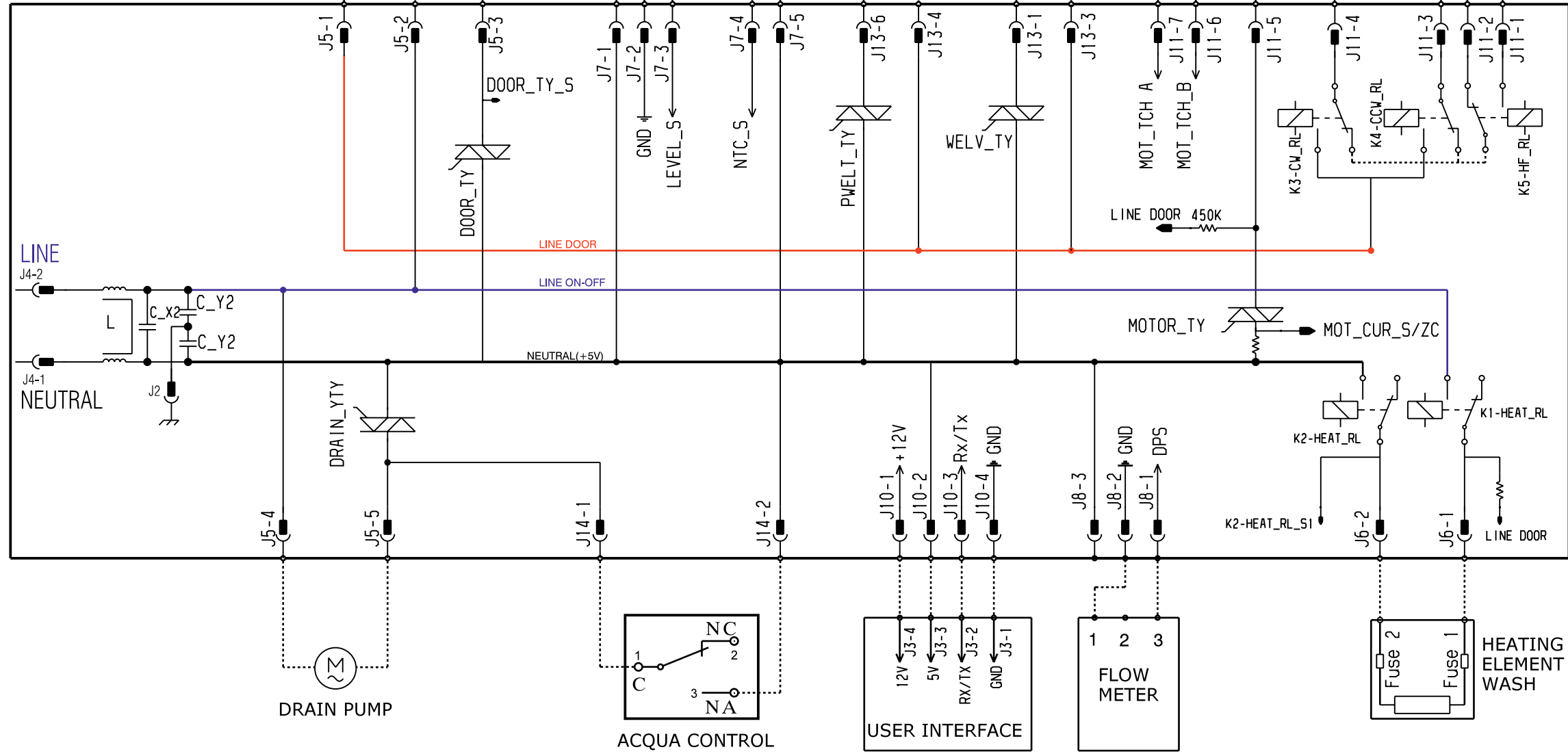
ELECTRIC DIAGRAM -EWM 09-
