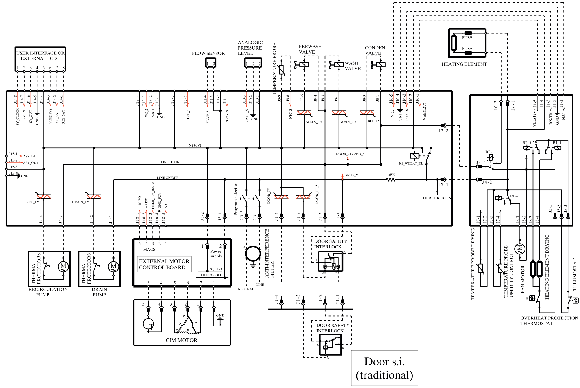
ELECTRIC DIAGRAM
