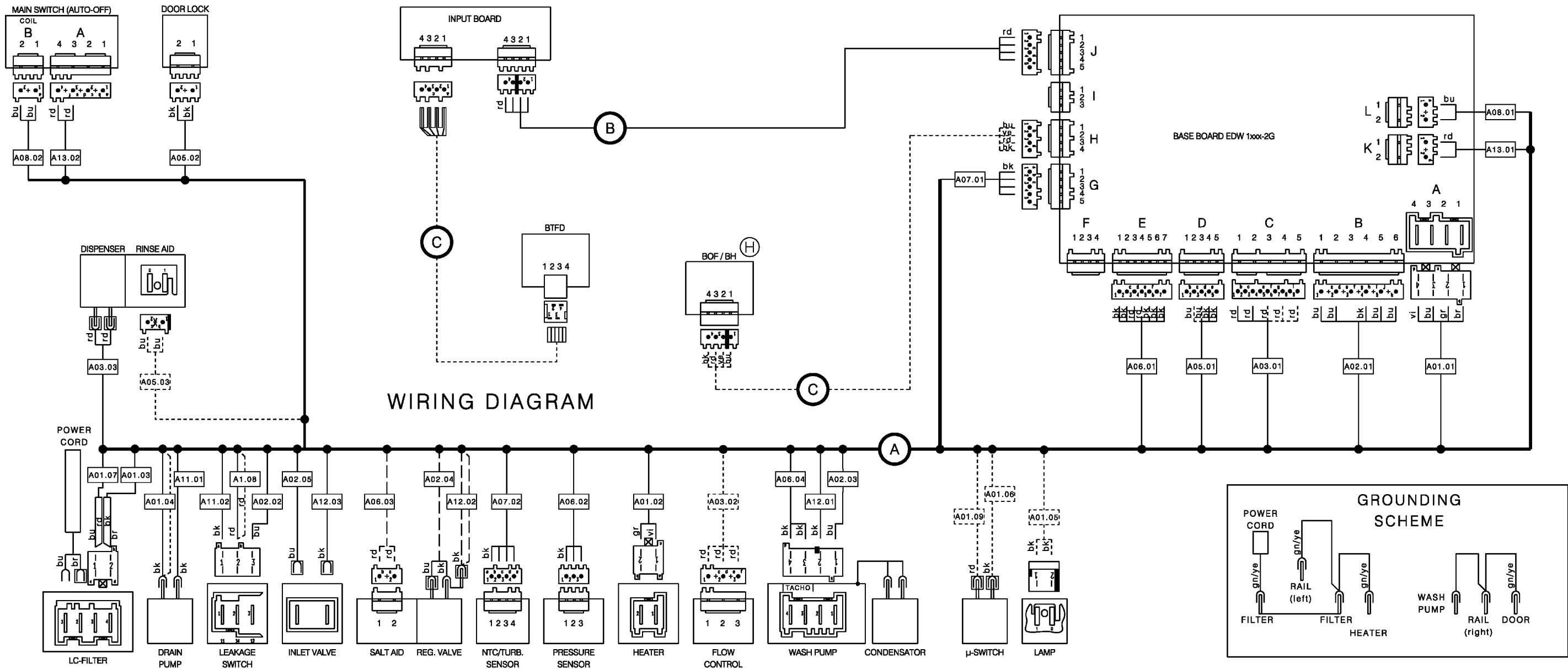
Connections included in WireHarnesses
