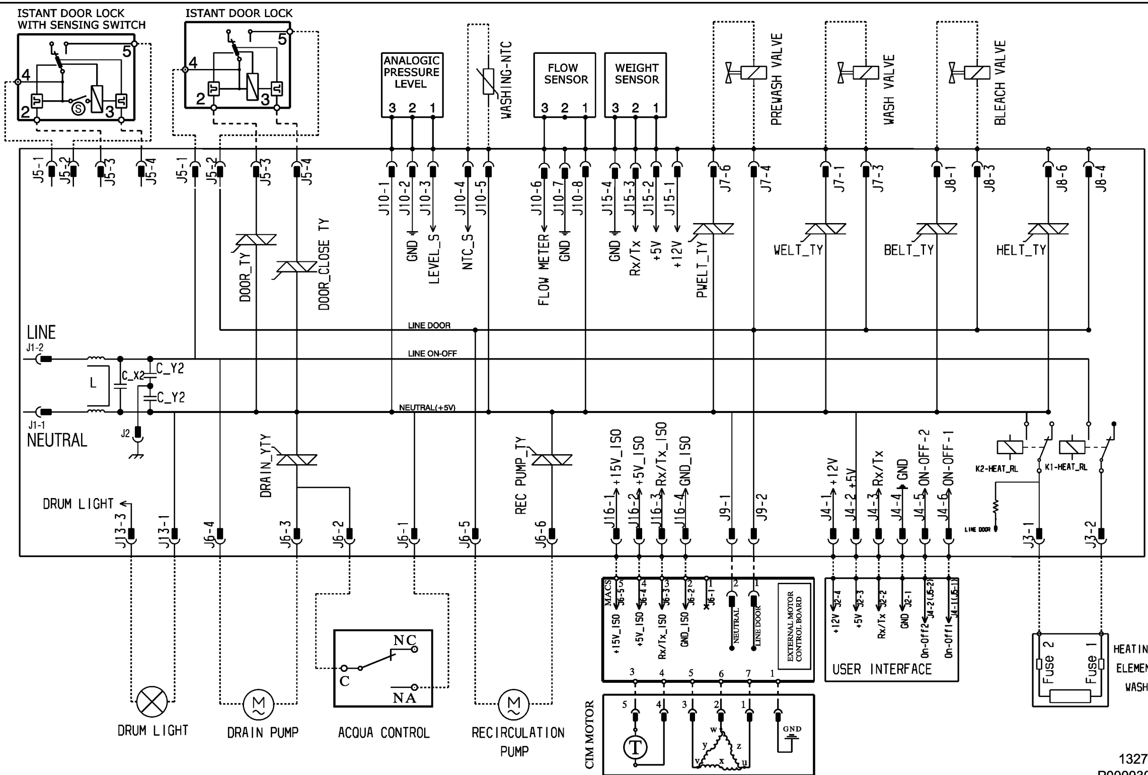
ELECTRIC DIAGRAM EWM10
