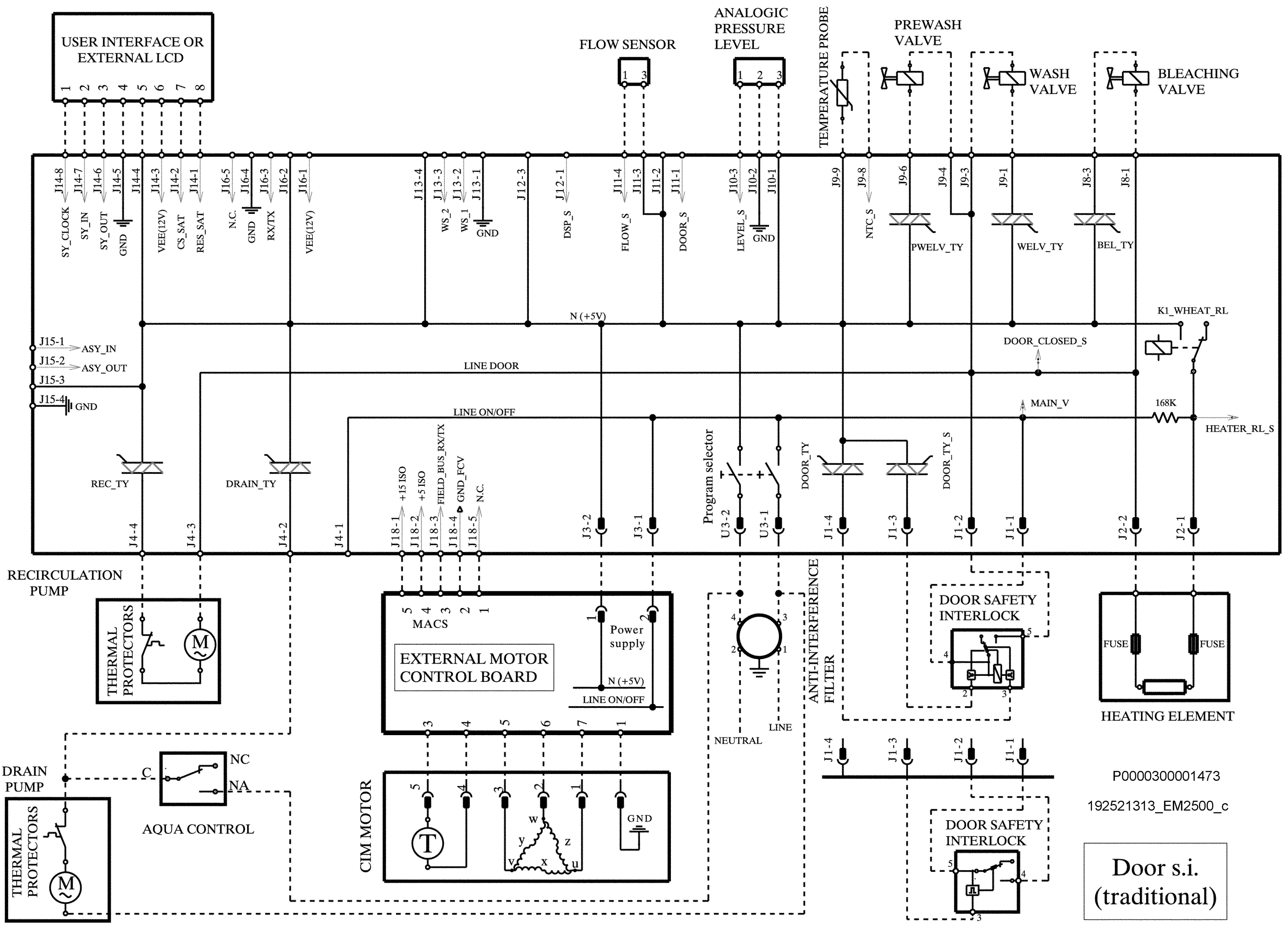
ELECTRIC DIAGRAM -
