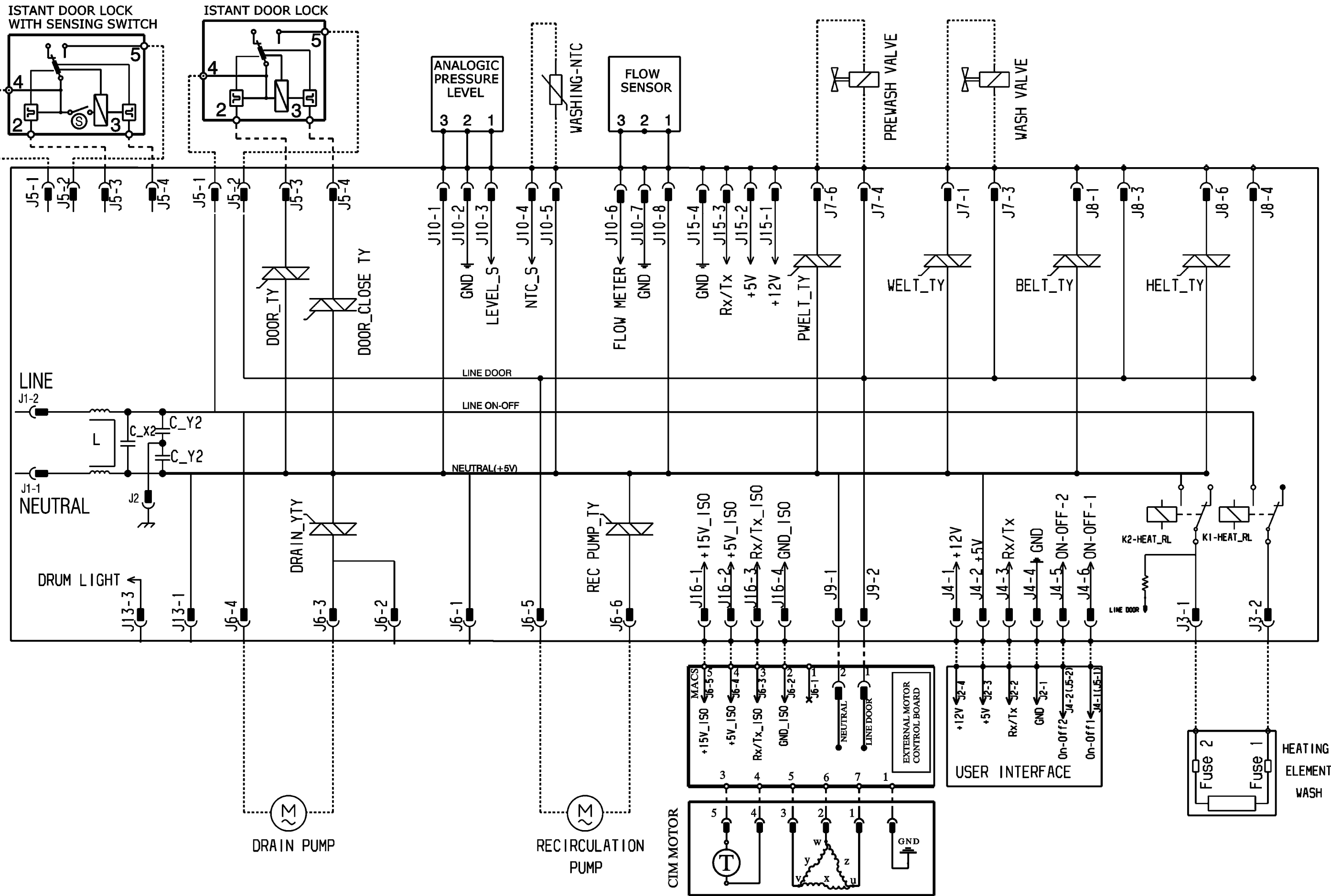
ELECTRIC DIAGRAM EWM10
