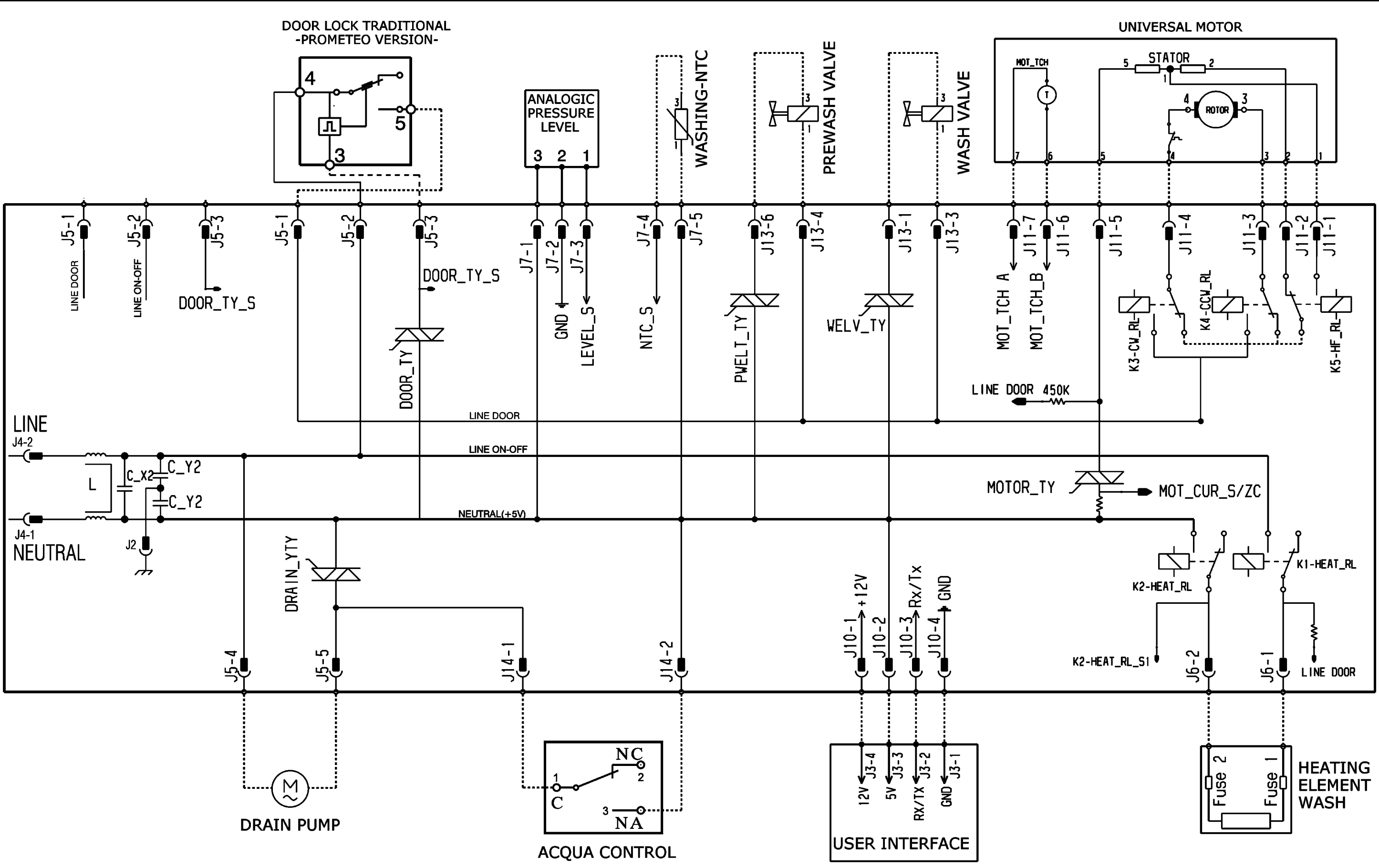
ELECTRIC DIAGRAM -EWM 09-
